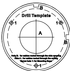
Figure 2-13 Drill Template of the Junction Box
