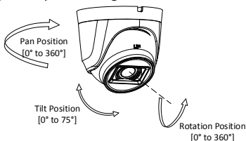
Figure 2-12 3-Axis Adjustment
