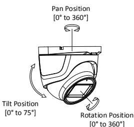
Figure 2-20 3-Aixs Adjustment
