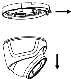
Figure 2-17 Remove the Mounting Base
