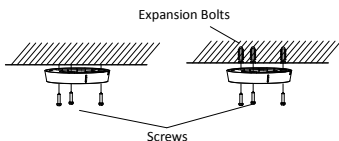
Figure 2-3 Attach the Mounting Base to the Ceiling
