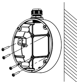
Figure 2-7 Secure the Junction Box on the Wall
