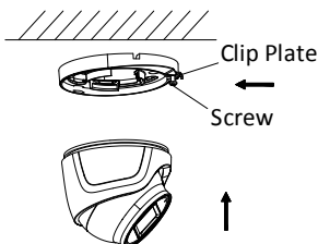
Figure 2-19 Secure the Camera
