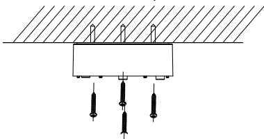
Figure 2-15 Secure the Junction Box on the Ceiling
