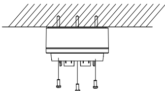
Figure 2-16 Combine the Junction Box's Cover back to its Body
